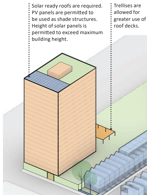
FIGURE 3.23: ROOF DESIGN
