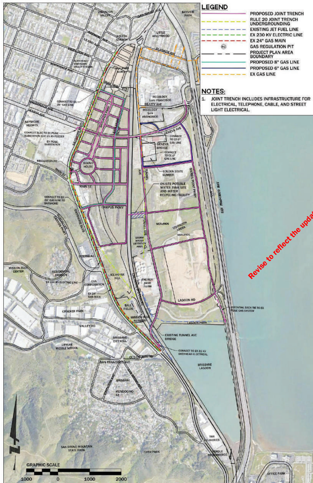
FIGURE 7.6 DRY UTILITIES AND KINDER MORGAN PIPELINES
